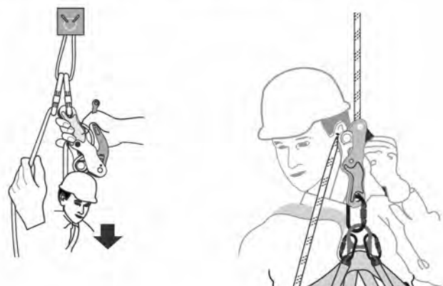
(b) RESCUE EVACUATION - From a Fixed Anchor-point
