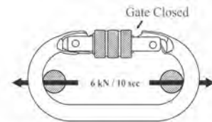
After the test, the gate shall open like new one. (Gate Function)
