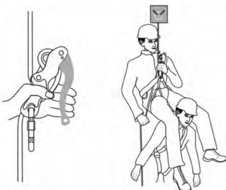
(a) RESCUE EVACUATION - Descent Assisted by Rescuer
