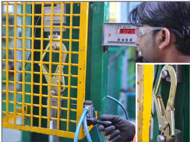
100 % proof load testing at 16 kN post assembly of components.
