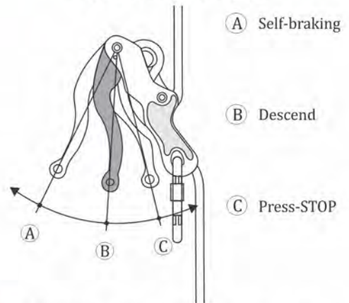
KARAM grip descender for positioning along with back up fall arrest system
