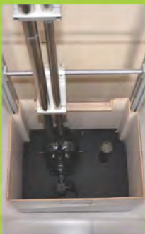
Drop Ball Impact Test
